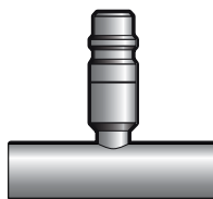
Quick-Disconnect Valve R-134a ONLY 13 mm – Low Side 16 mm – High Side
